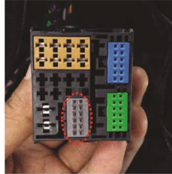
Pull out the GRAY connector.
