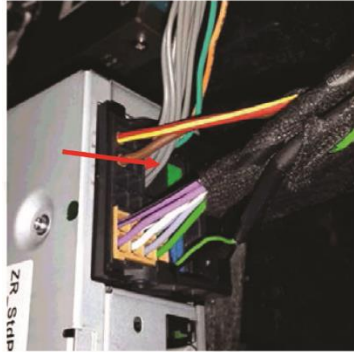
Unplug Quadlock connector.
