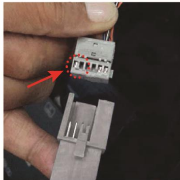
Plug the GRAY connector to the male GRAY connector of the PR-66K harness. Take note of the pin location. (circled)
