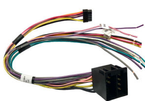
SWRSB-58 Harness
