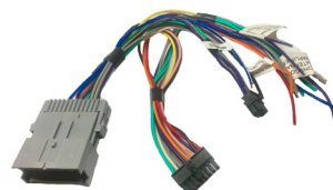
SOCGM-17C Harness
