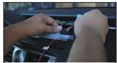
12. Make the power and LVDS connections on the factory screen.
