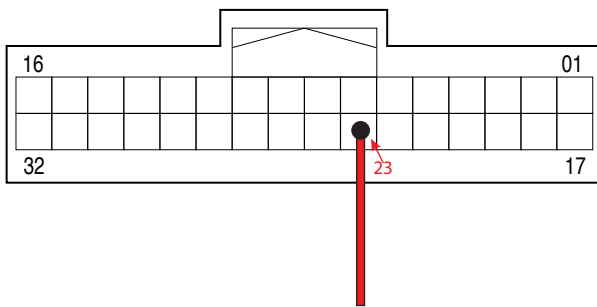
32 Pin Connector
