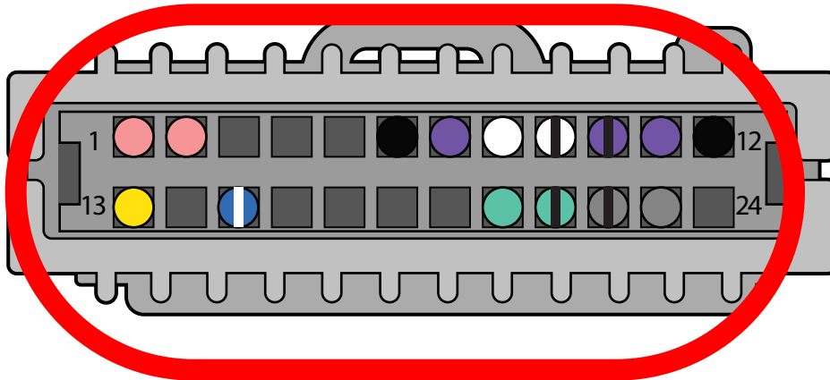
24 Pin Connector
