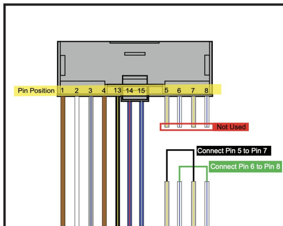
20 Pin Radio Display Connector (Top View)
